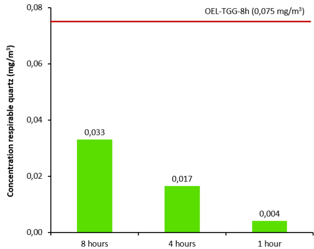
Figure 2. Test results for exposure respirable quartz relative to the OE
